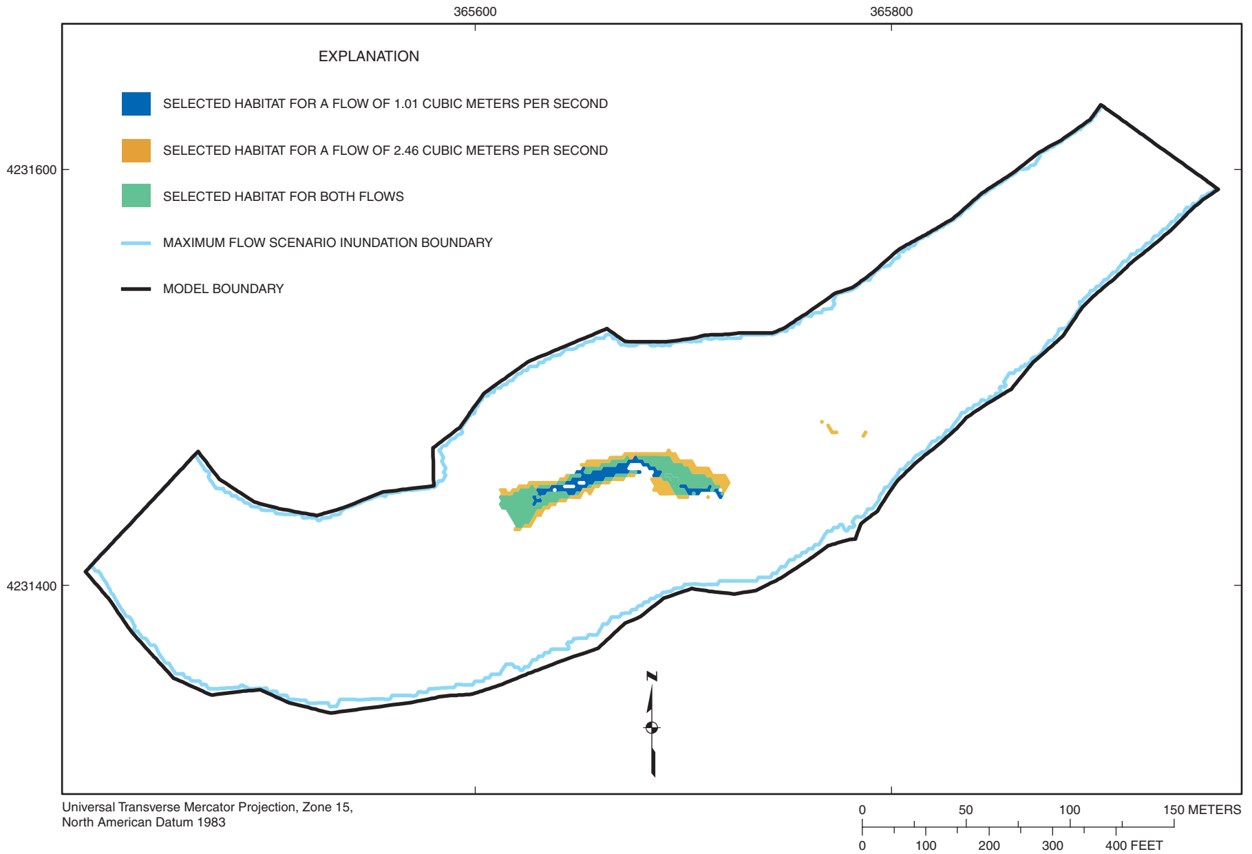
Figure 4-95. Selected habitat area distribution for habitat categories 24, 25 combined (stonecat) at flows of 1.01 and 2.46 cubic meters per second at Marais des Cygnes River site MDC2.
